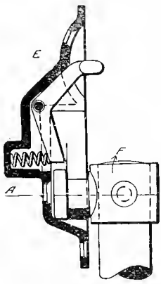
Fig. 3897. Section at Center.
